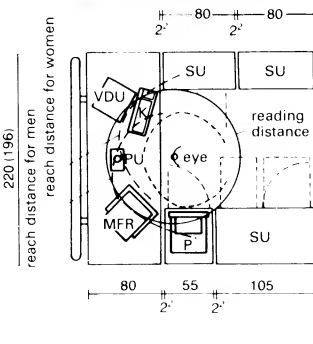
⑨ Plan view: workstation layout for open counters → ⑩ - ⑪
